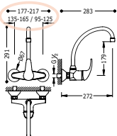
Monomando fregadero pared MONOTRES 2000
