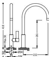
Monomando fregadero vertical CLASS
